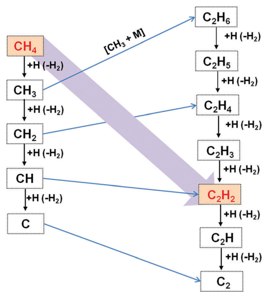
Fig. 2 H-shifting reaction sequences that drive the conversion of CH_4 to C_2H_2 and other CH_x ( x \leq 3 ) and C_2H_y ( y \leq 6 ) species in regions of high [H] and high T_{\text{gas}} .
