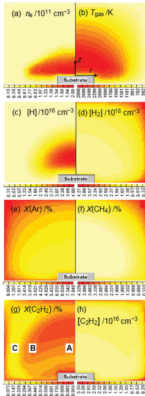
Fig. 4 Calculated 2-D( r, z ) distributions of (a) n_e , (b) T_{\text{gas}} , (c) [\text{H}] , (d) [\text{H}_2] , (e) X(\text{Ar}) , (f) X(\text{CH}_4) , (g) X(\text{C}_2\text{H}_2) and (h) [\text{C}_2\text{H}_2] for a MW activated gas mixture comprising F(\text{CH}_4) = 25 sccm, F(\text{Ar}) = 40 sccm, F(\text{H}_2) = 500 sccm, operating at p = 150 Torr and with P = 1.5 kW. The model assumes cylindrical symmetry, a reactor radius, r = 6 cm and height, h = 6.2 cm, and a substrate diameter of 3 cm.
