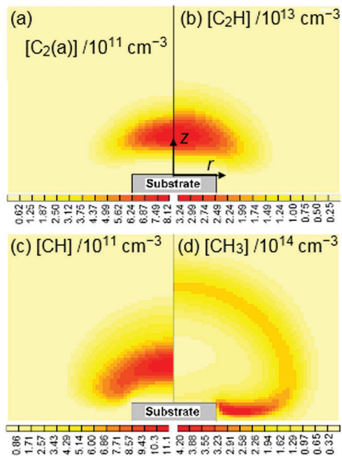
Fig. 6 Calculated 2-D( r, z ) distributions of (a) [C_2(a)] , (b) [C_2H] , (c) [CH] and (d) [CH_3] for the same reactor and operating conditions as in Fig. 4.
