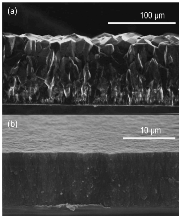
Fig. 1 Cross-section and tilt view scanning electron microscope (SEM) images illustrating (a) micro- and (b) nanocrystalline morphologies of CVD diamond films grown on Si substrates.
