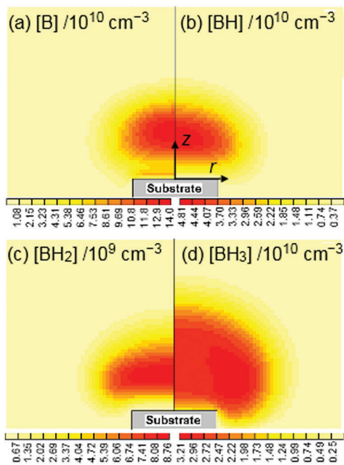
Fig. 7 Calculated 2-D( r, z ) distributions of (a) [B], (b) [BH], (c) [BH 2 ] and (d) [BH 3 ] in a MW activated gas mixture comprising F(\text{CH}_4) = 25 sccm, F(\text{Ar}) = 40 sccm, F(\text{H}_2) = 500 sccm, F(\text{B}_2\text{H}_6) = 0.009 sccm and F(\text{O}_2) = 0.006 sccm. All other details are as in Fig. 4.
