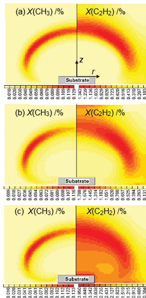
Fig. 9 Calculated 2-D( r, z ) mole fraction distributions X(\text{CH}_3) and X(\text{C}_2\text{H}_2) in a MW activated CH 4 /CO 2 /H 2 gas mixture comprising F(\text{CH}_4) = 350X_{\text{C}/\Sigma} sccm, F(\text{CO}_2) = 350(1 - X_{\text{C}/\Sigma}) sccm and F(\text{H}_2) = 150 sccm, with p = 150 Torr, P = 1 kW and X_{\text{C}/\Sigma} = (a) 0.47, (b) 0.5 and (c) 0.54. The reactor dimensions for the modelling are the same as in Fig. 4.
