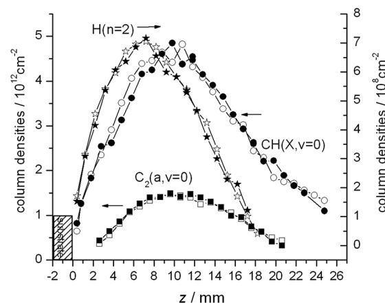
Fig. 5 Comparison of \text{C}_2(a, v=0) and \text{CH}(X, v=0) radical (left hand scale) and \text{H}(n=2) atom (right hand scale) column densities measured by CRDS as a function of height ( z ) above the substrate surface in the same MW CVD reactor, operating at the same p (150 Torr) and P (1.5 kW), using the following gas mixtures: (i) F(\text{CH}_4) = 25 sccm, F(\text{Ar}) = 40 sccm, F(\text{H}_2) = 500 sccm and (ii) F(\text{C}_2\text{H}_2) = 12.5 sccm, F(\text{Ar}) = 40 sccm, F(\text{H}_2) = 512.5 sccm (filled and open symbols, respectively).
