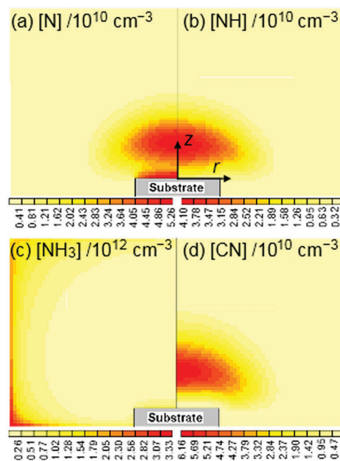
Fig. 8 Calculated 2-D( r, z ) distributions of (a) [N], (b) [NH], (c) [NH 3 ] and (d) [CN] in a MW activated gas mixture comprising F(\text{CH}_4) = 20 sccm, F(\text{N}_2) = 3 sccm and F(\text{H}_2) = 477 sccm, with all other details as in Fig. 4.
