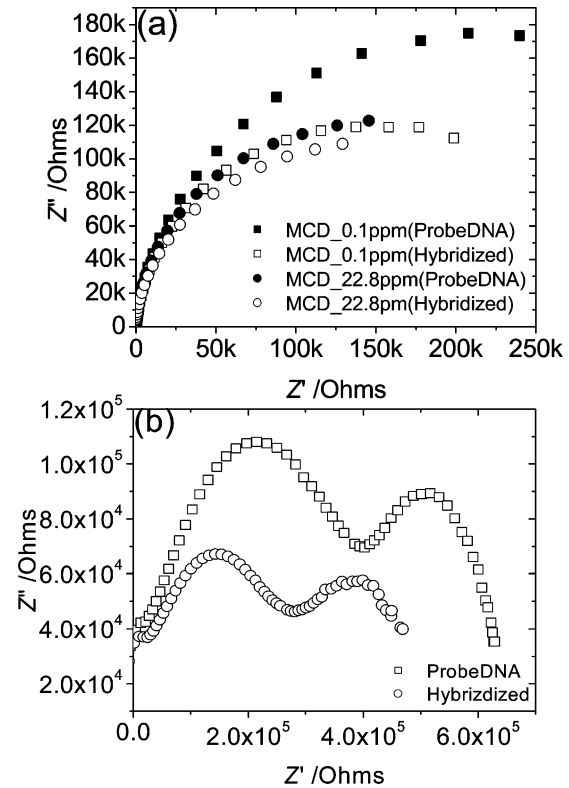
Figure 10. DNA sensing: (a) Nyquist plot of probe DNA immobilized (shaded) and after hybridization to complimentary target DNA (voided) on MCD_0.1 ppm (■) and MCD_22.8 ppm (●); (b) Nyquist plot of probe DNA immobilized on undoped MCD (■) and after hybridization to complimentary target DNA (●).
