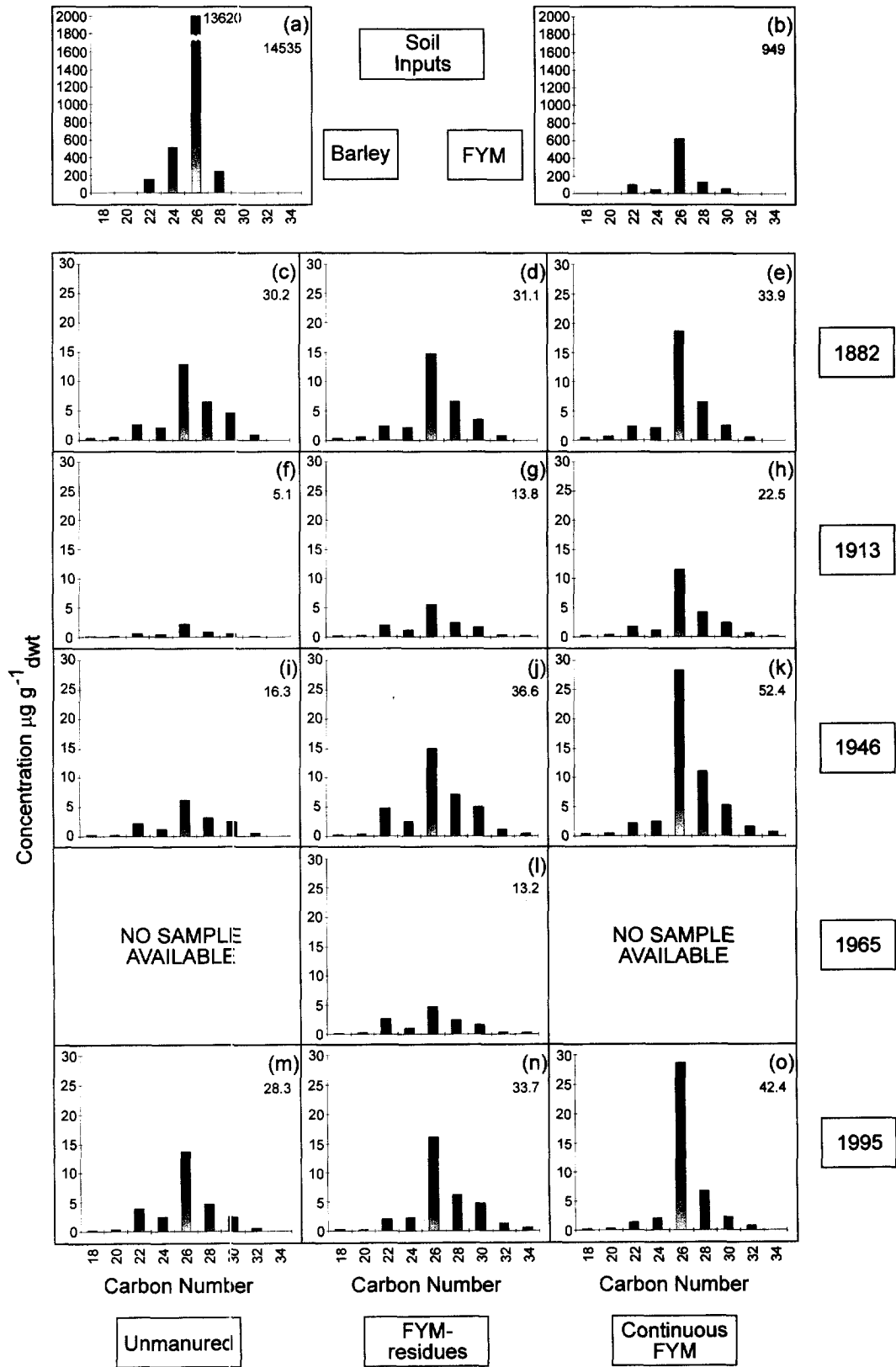
Fig. 2. Distributions for the major n -alkanol components detected in the inputs and soil samples. Each column relates to a different series whilst each row corresponds to a specific sampling year. The value below each figure letter, (a) to (o), denotes total abundance ( \mu\text{g g}^{-1} soil dwt).
