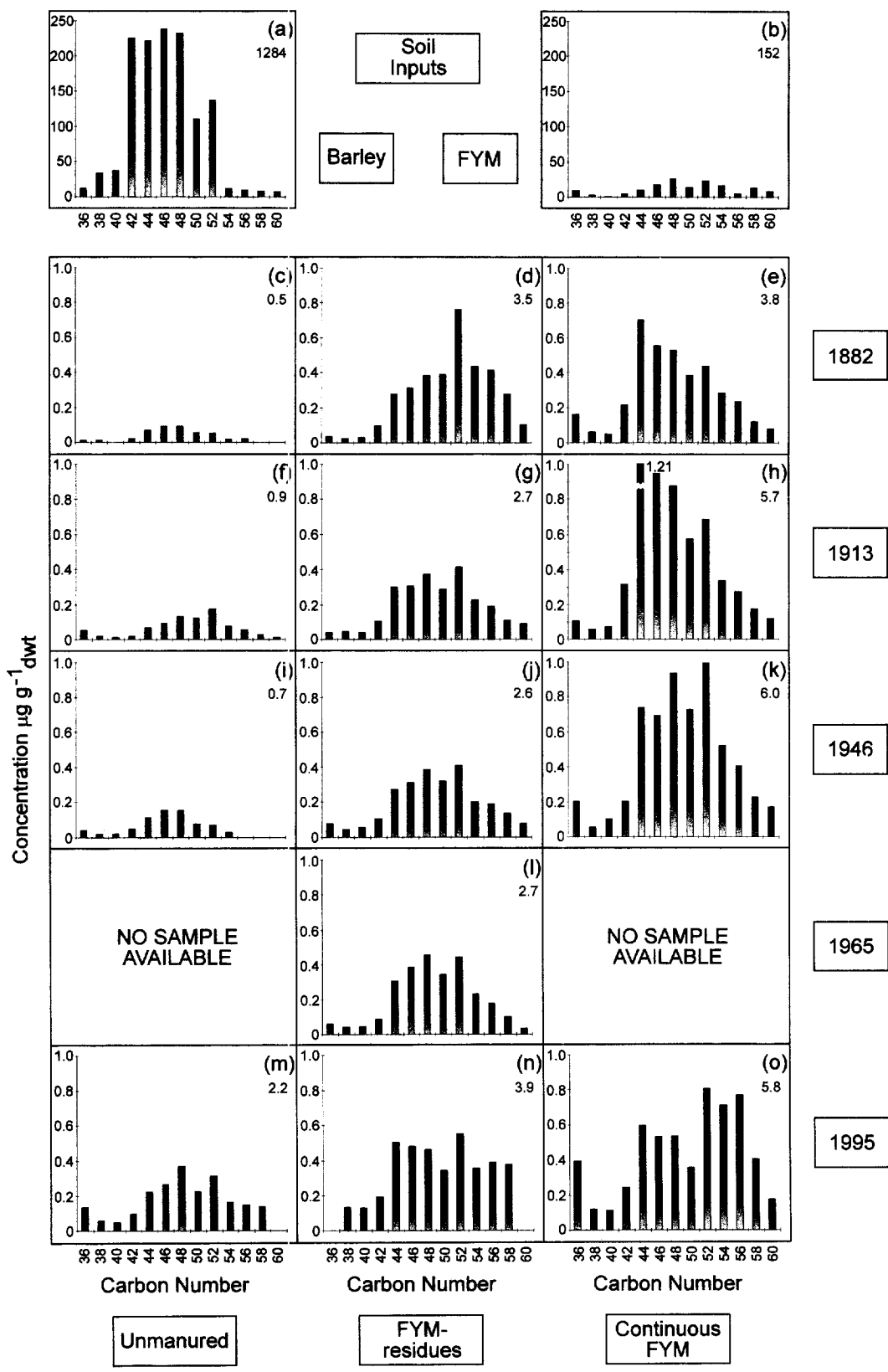
Fig. 1. Distributions for the major wax ester components detected in the inputs and soil samples. Each column relates to a different treatments whilst each row corresponds to a specific sampling year. The value below each figure letter, (a) to (o), denotes total abundance ( \mu\text{g g}^{-1} soil dwt).
