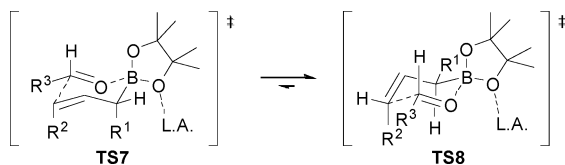
Figure 2. Stereoselectivity of ( Z )-allylic-boronic esters.
