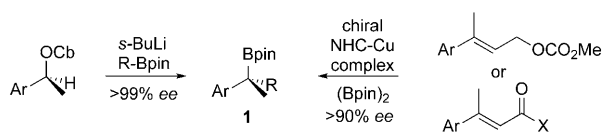
Scheme 1. Synthesis of chiral tertiary boronic esters. Cb = N,N -diisopropylcarbamoyl, Bpin = pinacolboronyl, NHC = N -heterocyclic carbene.
