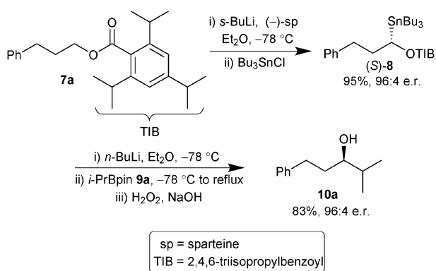
Scheme 2 Preparation of 2,4,6-triisopropylbenzoates and homologation of boronic esters.
