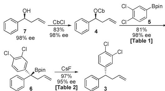
Scheme 2. Synthesis of Olefin 3 via Lithiation/Borylation–Protodeboration Sequence a
