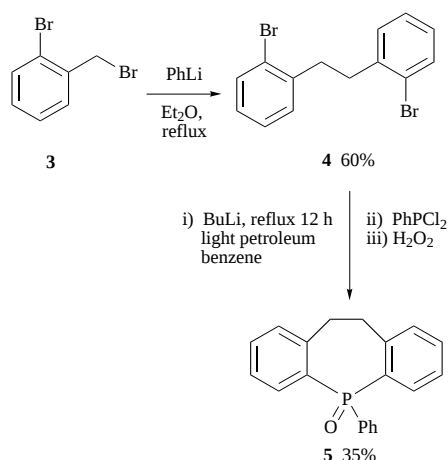
Scheme 1
