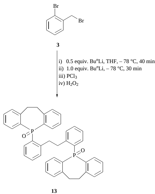
Scheme 5
