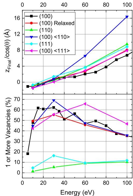
Fig. 7. Results from repeated simulations of deuterium bombardment various diamond surfaces at 300 K. Where only a surface is specified in legend, bombarding atoms were at an incident angle of 0^\circ . Directions indicated correspond to implantation angles upon a (100) surface. (110), (111), and (100) relaxed were all constructed by applying a rotation matrix to a larger block of diamond, trimming it to size, and performing an energy minimization. The depth plotted takes into account the incident angle, \theta , effectively plotting the distance traveled within the diamond rather than depth, z_{\text{final}} .
