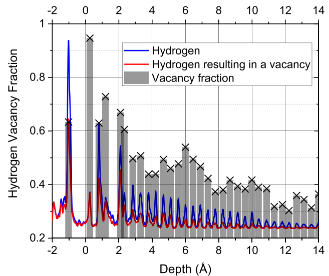
Fig. 4. Fraction of hydrogen that caused one or more vacancies compared with all implanted hydrogen as a function of depth for all simulations of a (100) surface. Blue line shows the density of hydrogen depths, and the red line also shows this but only for hydrogen that resulted in one of more vacancies forming. The black bars show the ratio between two densities for the hydrogen peaks.
