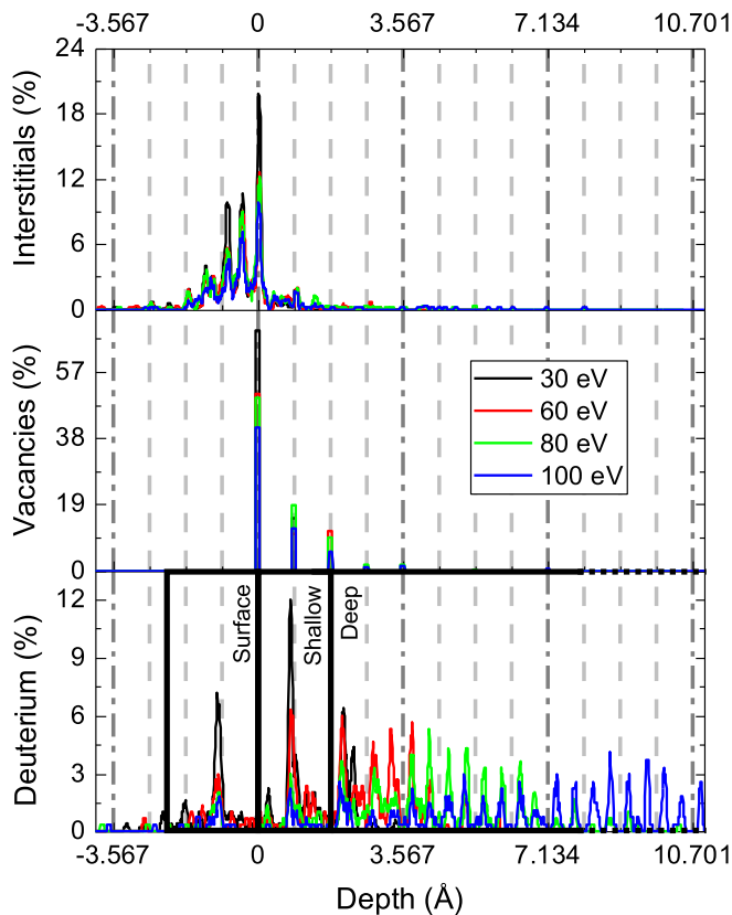
Fig. 3. Defect analysis of four datasets of 300 repeats of a (100) diamond block at 300 K being bombarded with a single deuterium atom of 30, 60, 80, and 100 eV normal to the surface. y-axis units are as a percentage of incident atoms (for example, 39% of incident atoms caused a vacancy in the top AL for 100 eV). Interstitials are the depth of any carbon atom with an occupancy of two, meaning each vacant site will result in two interstitials provided no carbon is lost. The percentage was halved to account for this. Dashed lines show the ALs of the diamond, with markers at every UC. Three depth categories ( surface , shallow , and deep ) were used for discussion as marked on the deuterium density plot.
