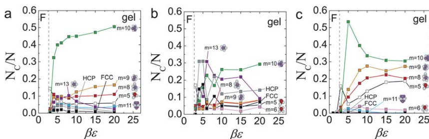
Fig. 5 The effect of quench rates on the local structure in polydisperse systems. (a) TCC analysis for a quench time of 671 \tau_B . (b) TCC analysis for a quench time of 1.01 \times 10^4 \tau_B . (c) Data from an instantaneous quench. Dashed lines denote \epsilon^c .
